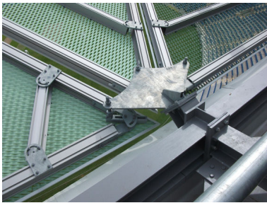
Garston architectural expanded metal installed as rain screen cladding at Carnegie Pavilion, Headingley Cricket Ground, Leeds, England.
